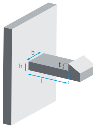
Figure 11. Snap-fit geometry
