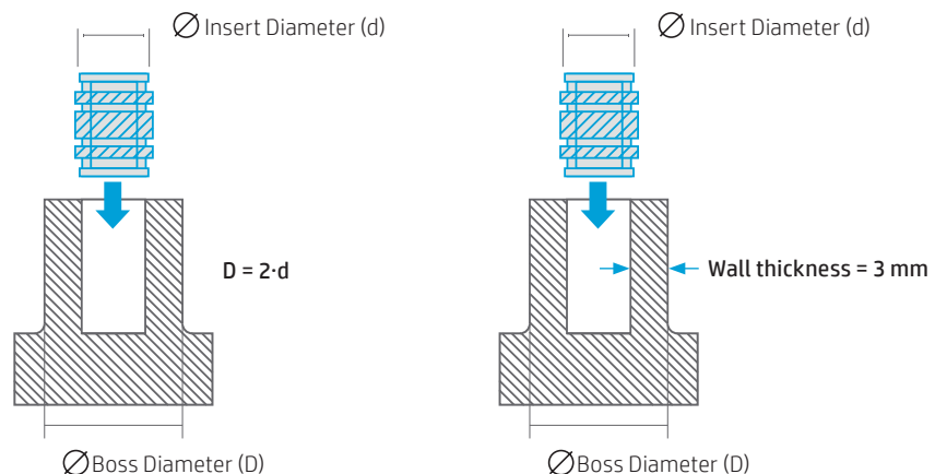
Figure 2: Boss diameter
